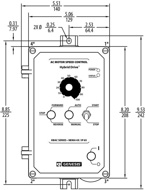
Figure 5 – Model KBAC-24D Mechanical Specifications (Inches/mm)
