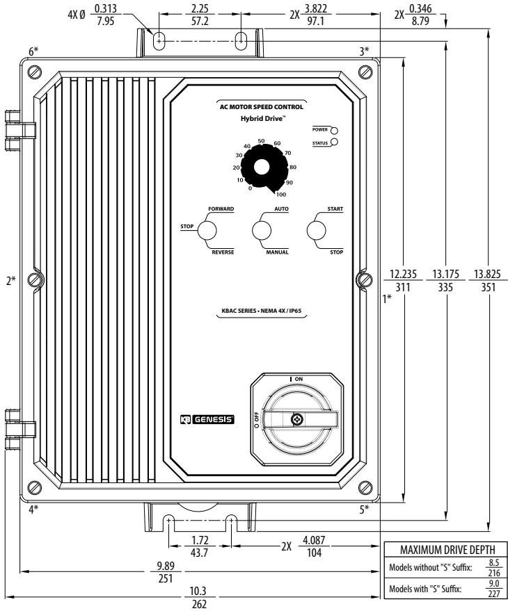
Figure 7 – KBAC-217, 416 Series Mechanical Specifications (Inches/mm)
