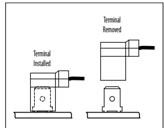
Figure 21 – Removing Jumper J1 on Models KBAC-24D, 27D
