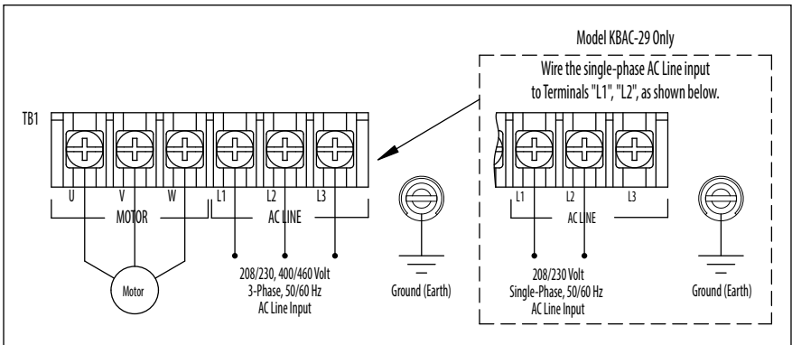
Figure 11 – Models KBAC-29*, 45, 48 AC Line Input, Motor, and Ground Connections
