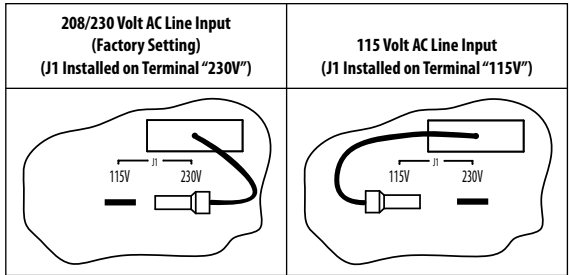
Figure 20 – Models KBAC-24D*, 27D AC Line Input Voltage Selection
