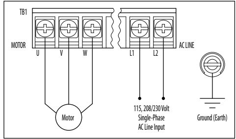
Figure 10 – Models KBAC- 24D, 27D*, 29 (1P) AC Line Input, Motor, and Ground Connections
