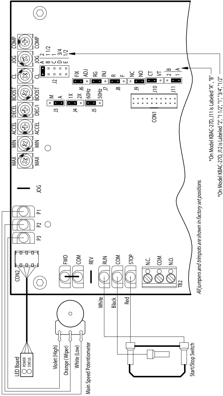
Figure 3 – KBAC-27D*, 29, 29 (1P), 45, 48 Control Layout 1
