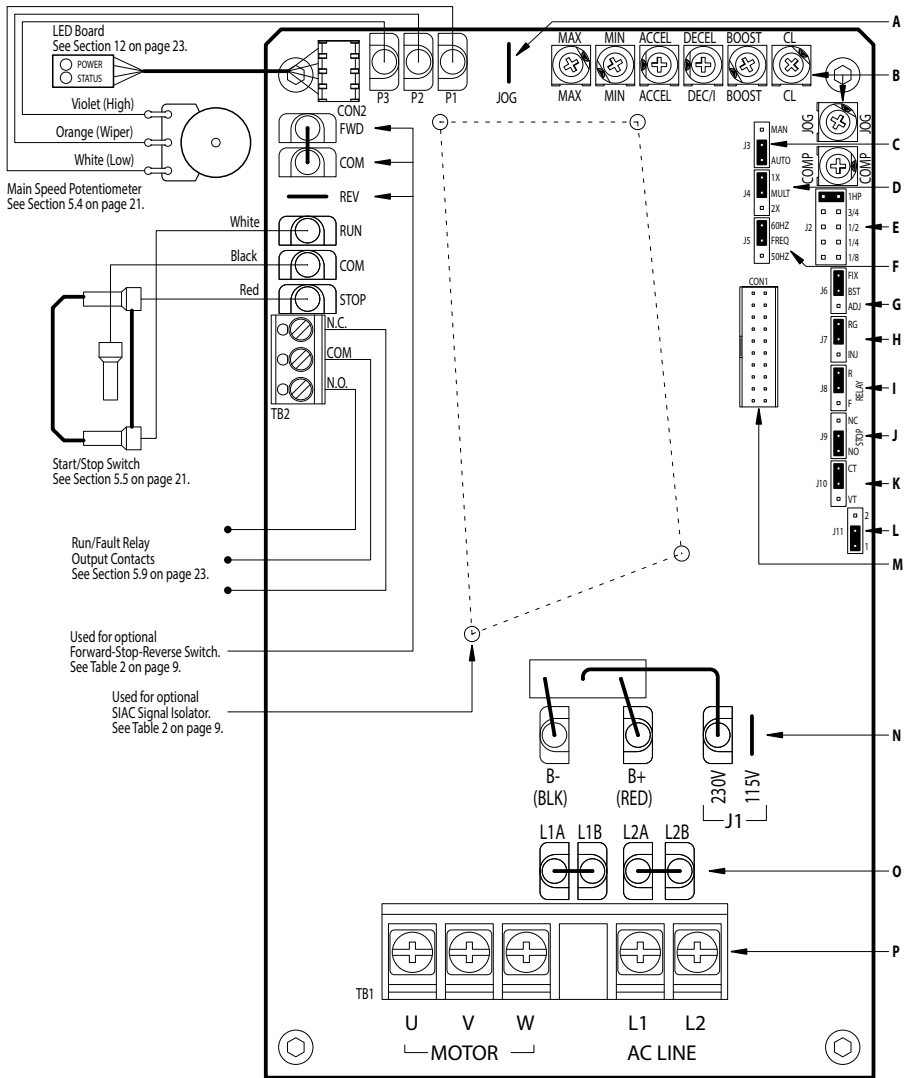
Figure 2 – KBAC-24D Control Layout
