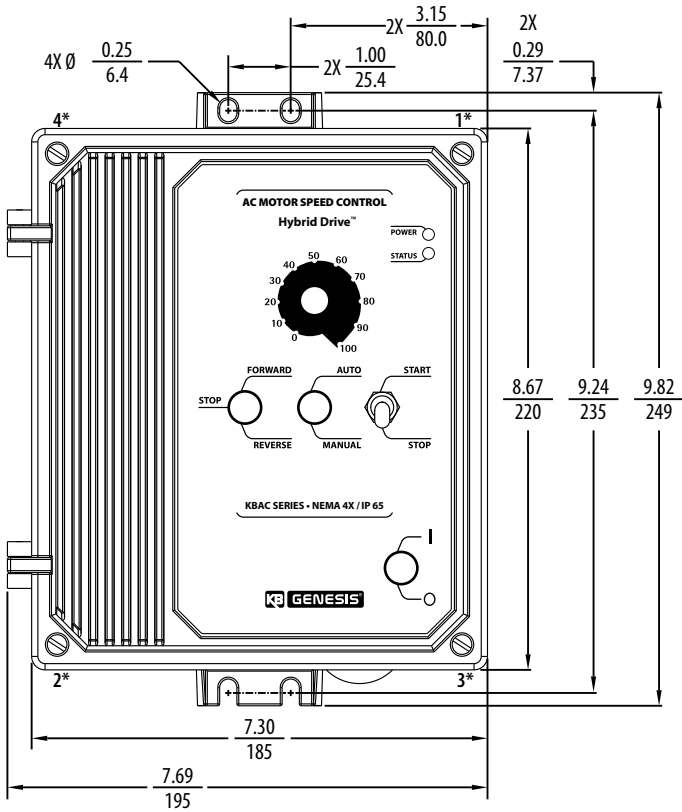
Figure 6 – Models KBAC-27D, 29, 29 (1P), 45, 48 Mechanical Specifications (Inches/mm)
