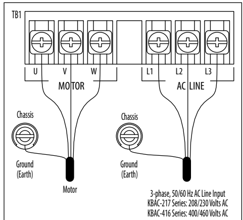
Figure 12 – KBAC-217, 416 Series AC Line Input, Motor, and Ground Connections
