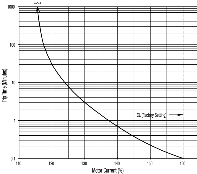
Figure 41 – I t Trip Time vs. Motor Current
